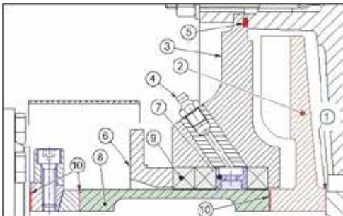
Figure 4: Expeller gland
