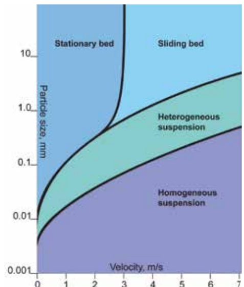
Figure 1: Example of flow configurations (sand density = 2700\text{ kg/m}^3 , pipe diameter = 160\text{ mm} )
