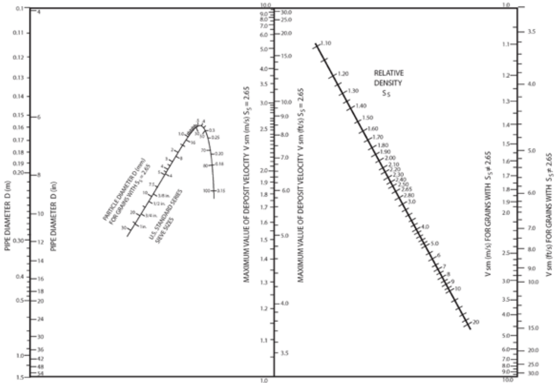
Nomographic chart for minimum velocity. (Adapted from Wilson, 1976).
