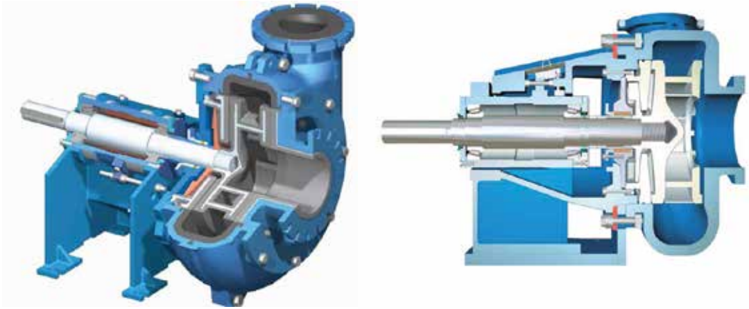
HR wet end single adjust, HM wet end double adjust
