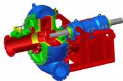
Sectional view of a Metso Outotec dredge pump
