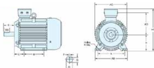
IEC foot mounted motor with overhead mounted terminal box
