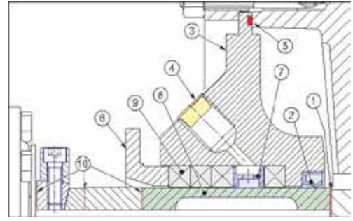
Figure 2: Low flow gland
