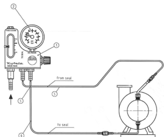
Figure 14: Example of a high pressure flush system
