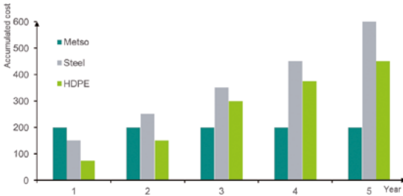
Figure 4: A cost comparison between Metso Outotec, conventional steel pipes and HDPE, based on the following operational date: 2 lines with total length of approx. 100ft (300m) having an inside diameter of 6 in. (152 mm) for carrying slurry (35% solid material of diabase and gneiss with a particle size up to 3/16 in. (5mm) Working pressure 75 psi (5kp/cm 2 ). Flow rate 11 ft/sec (3.3 m/s). Capacity 140 000 tons of solid material per year.
