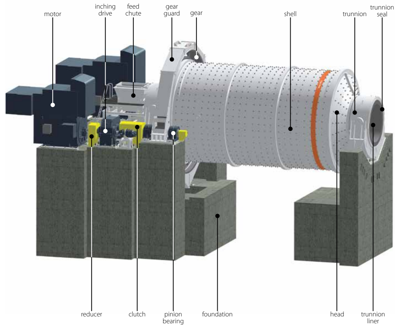
Illustrative example of components covered by engineered to order solutions in a ball mill.
